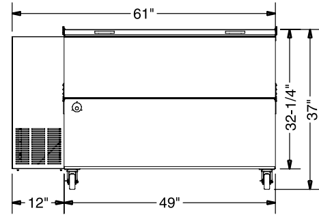
MCATS-122S ELEVATION VIEW
