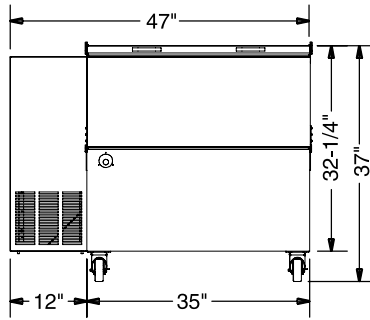
MCATS-082S ELEVATION VIEW
