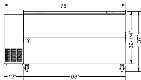
MCATS-082S ELEVATION VIEW
